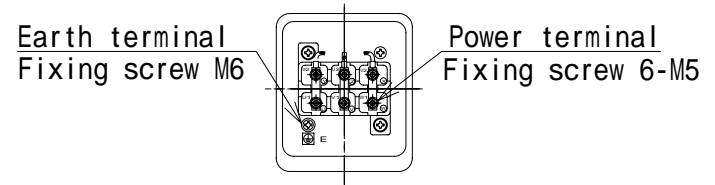
Detail of terminal box
